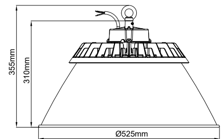
Tall Reflector
